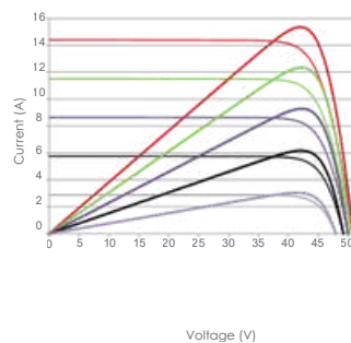
Current-Voltage & Power-Voltage Curves (575W)
